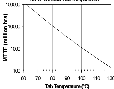
MTTF vs. GND Tab Temperature
